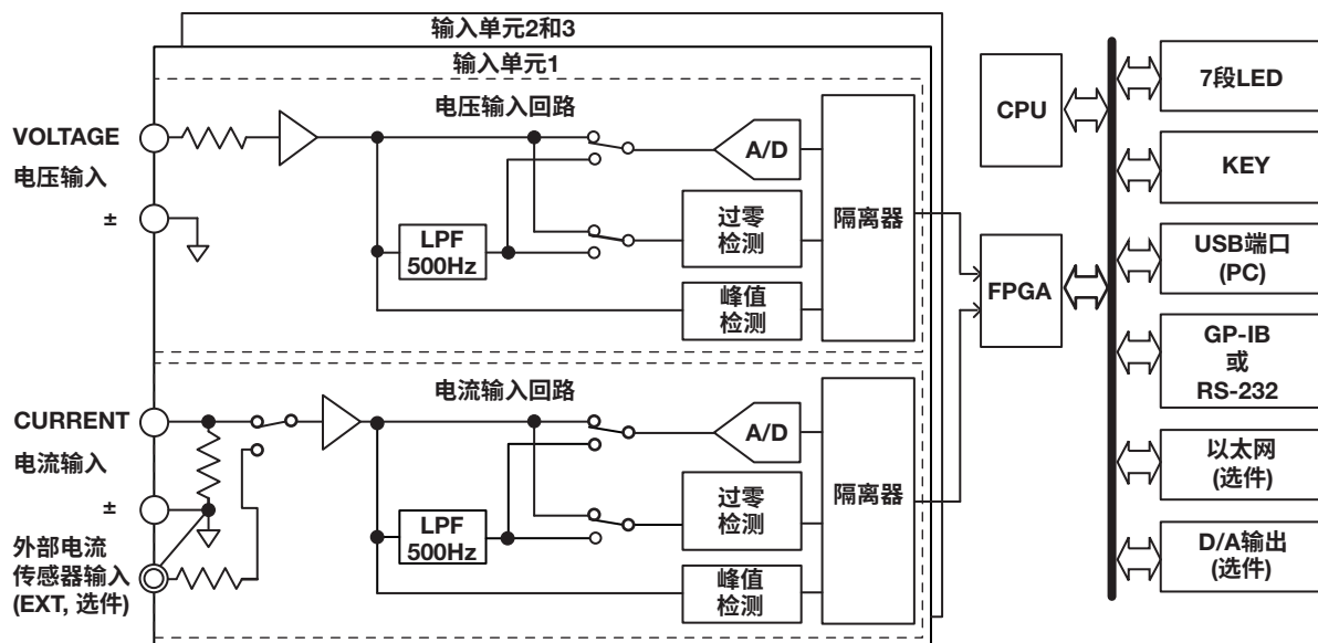
WT310E电流输入(CURRENT INPUT)
