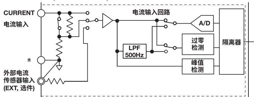
WT310E电流输入(CURRENT INPUT)
