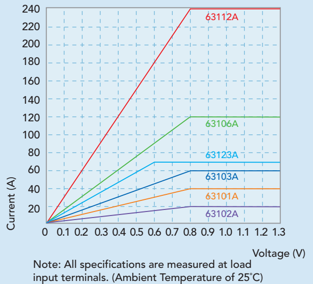
低电压特性 (Typical) 型号 63101A/63102A/63103A/63106A/63112A/63123A
