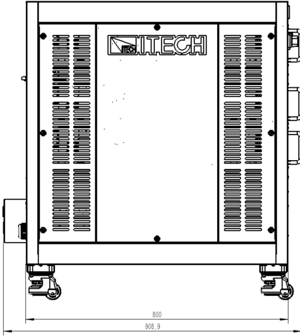
IT7984E-350-360/IT78105E-350-450/ IT78126E-350-540
