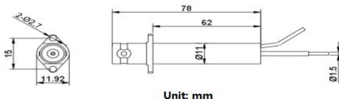
(CSD050A, CSD100A 机械规格)
