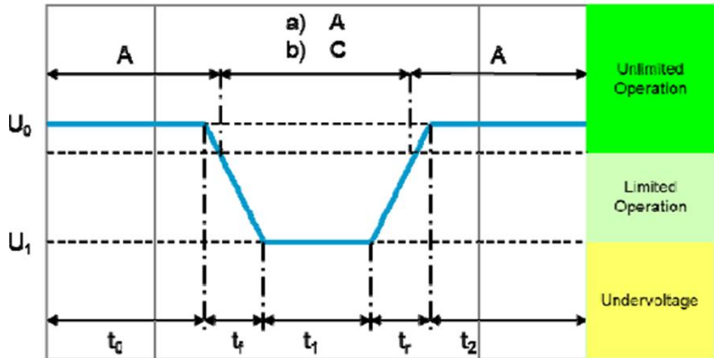
E-15 Test pulse parameters for E48-10 Starting pulses
